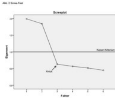
Abb. 2 Scree-Test
